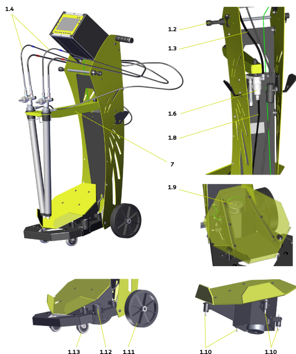
Chariot Inocart VT Dual Europe / US
